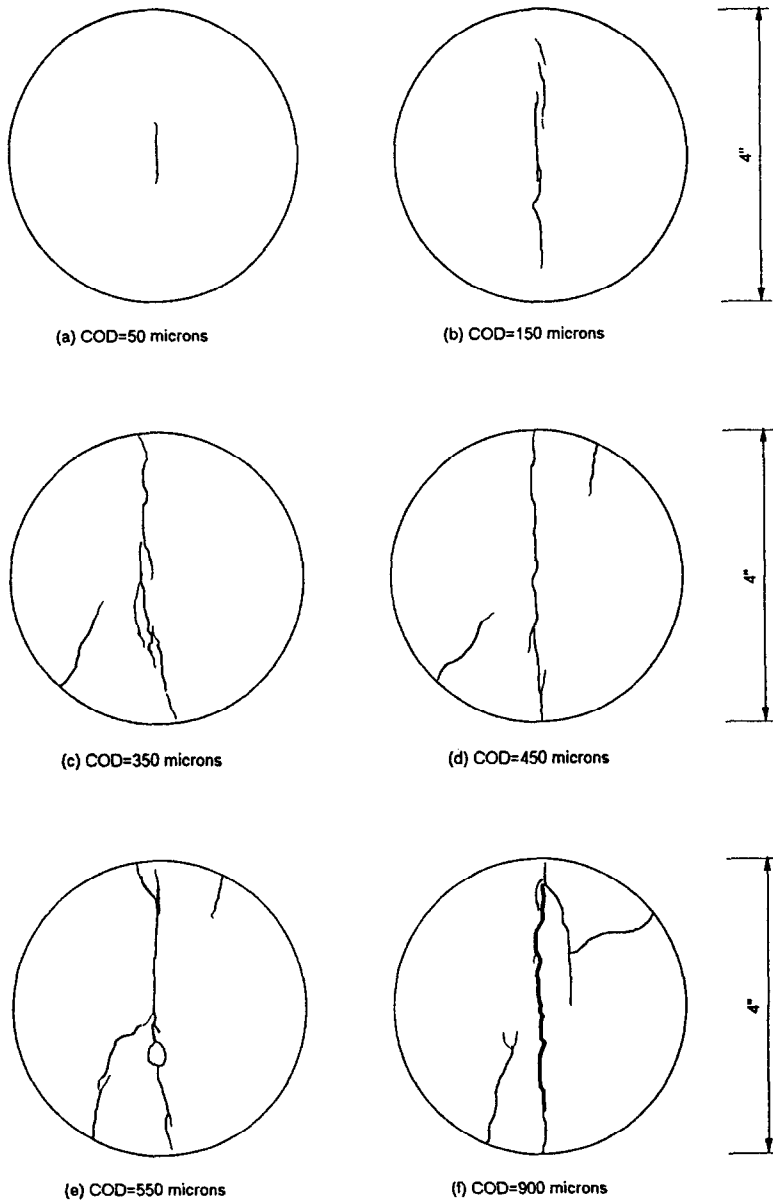
FIG. 6. Crack patterns.
